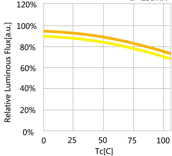
Case Temperature vs. Relative Luminous Flux If=150mA
