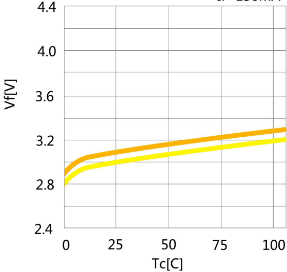
Case Temperature vs. Forward Voltage If=150mA
